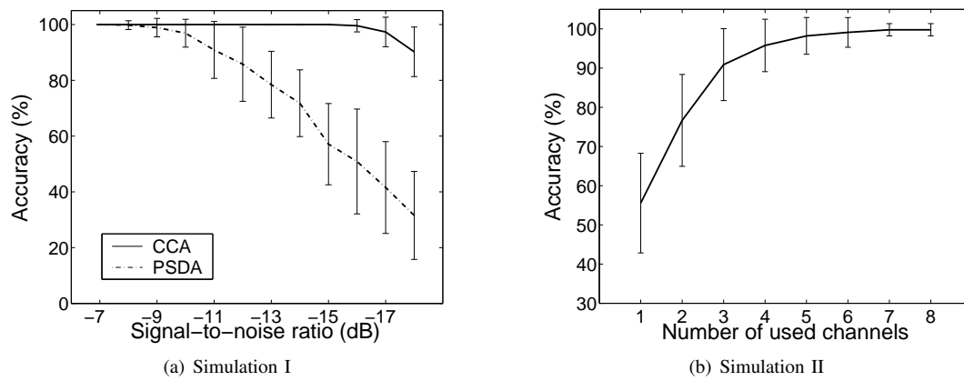
Fig. 2. The influence of noise on the two recognition approach (Fig. 2(a)) and the influence of number of channel on the CCA approach (Fig. 2(b), the SNR is -15 dB) were studied by simulation. The error bars represent standard deviations. Fig. 2(a) shows that the CCA approach is more robust than the PSDA approach. Fig. 2(b) shows that using more channels for the CCA approach may improve recognition accuracy.
